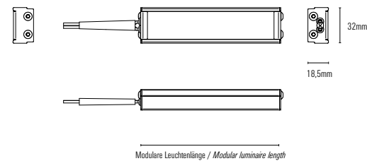
SKIZZE ACR FOODLIGHT-HT: DIAGRAM OF ACR FOODLIGHT-HT:
